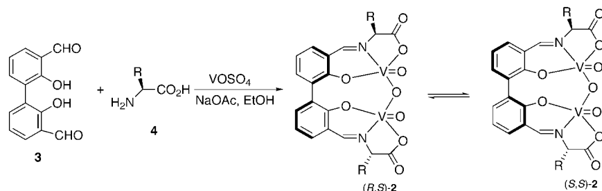
Scheme 2. Preparation of catalysts 2 .
